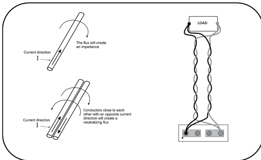
(Figure 6) Avoid Loops or “windows”. When resistance is low, the major part of the impedance is caused by the reactance. Minimizing the magnetic flux will reduce the reactance. Cables of opposing currents can be twisted together over the length of the cable to minimize the flux.
