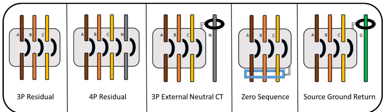
(Figure 1) Ground Fault Detection Methods on Low Voltage Circuit Breakers. 3 Pole Residual, 4 Pole Residual, 3 Pole Residual with External Neutral CT, Zero Sequence, and Source Ground Return.
